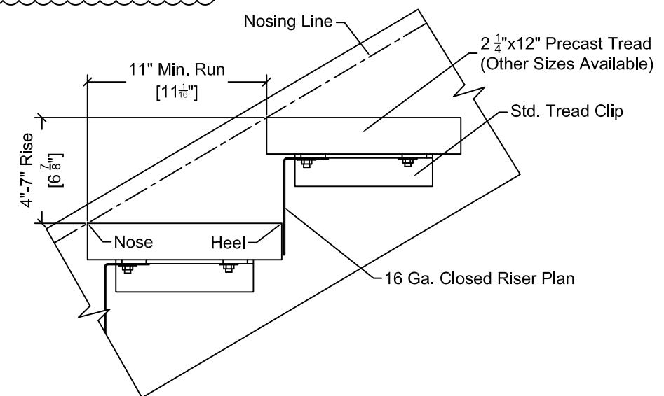
Detail A
